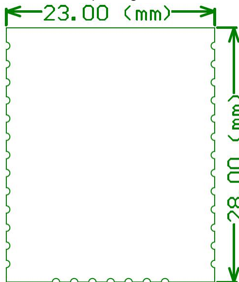
Figure 4-1 package outline drawing
